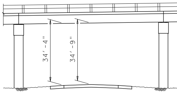
Highway 34' - 4" beneath Structure
