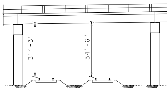
Railroad 31'-3" beneath Structure
