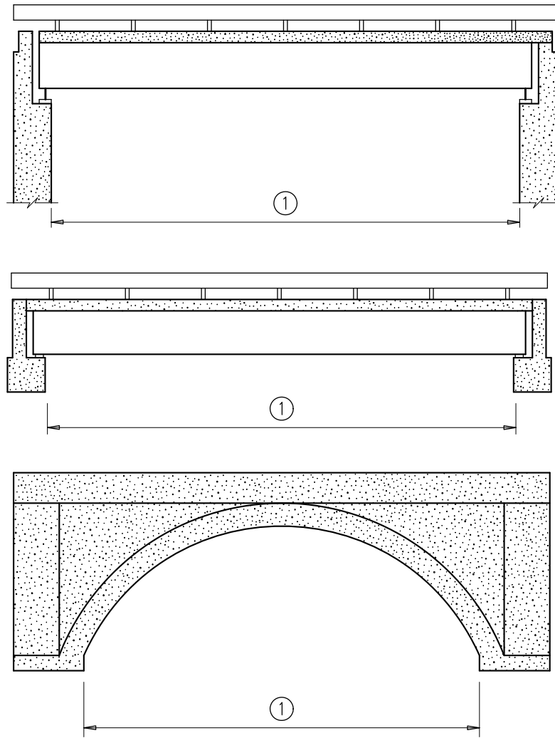
① Item 112 ~ NBIS Bridge Length
