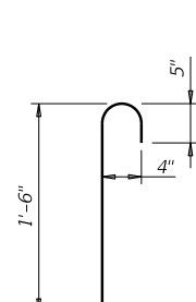
BARS CS (Length = 2'-3")
