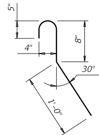
BARS CL (Length = 2'-5")
