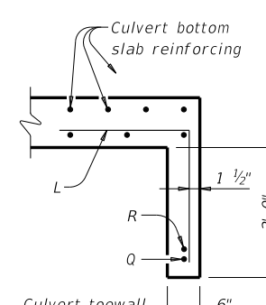
SECTION B-B (5)
