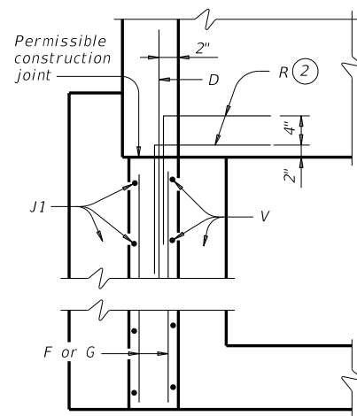
WINGWALL
