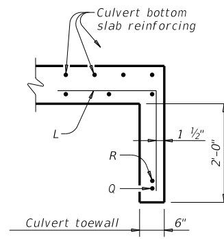
SECTION B-B (5)
