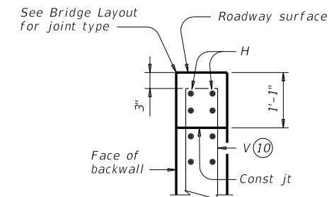
BACKWALL DETAIL
