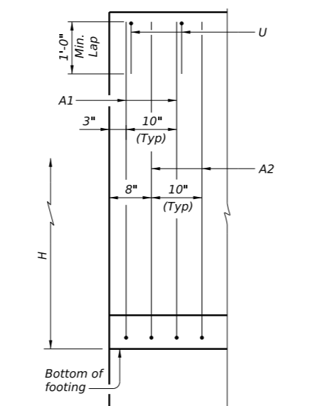
PARTIAL WALL ELEVATION (Showing vertical reinforcing pattern in back face.)
