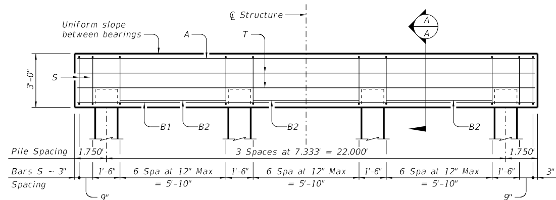
ELEVATION ③ ⑤ (4 Pile bent)
