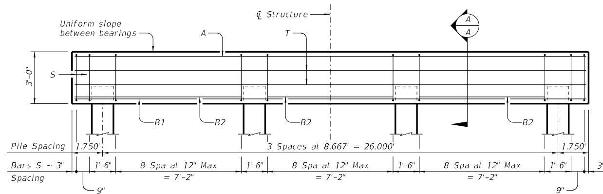
ELEVATION ③ ⑤ (4 Pile bent)
