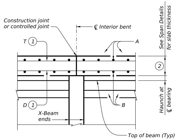
SECTION A-A Bars OA (Top) not shown for clarity.
