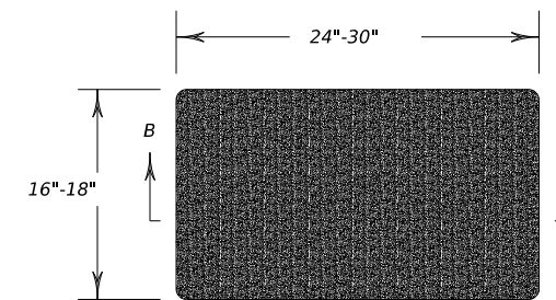
SANDBAG DETAIL
