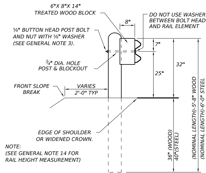
TYPICAL POST PLACEMENT
