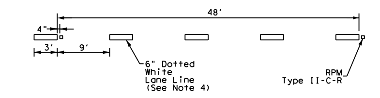
DETAIL C
