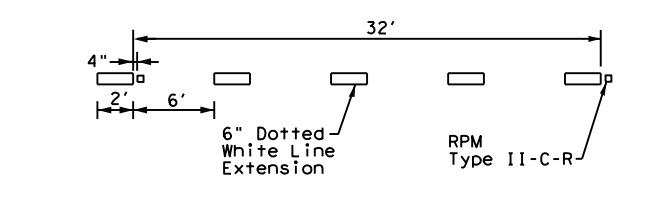
DETAIL D
