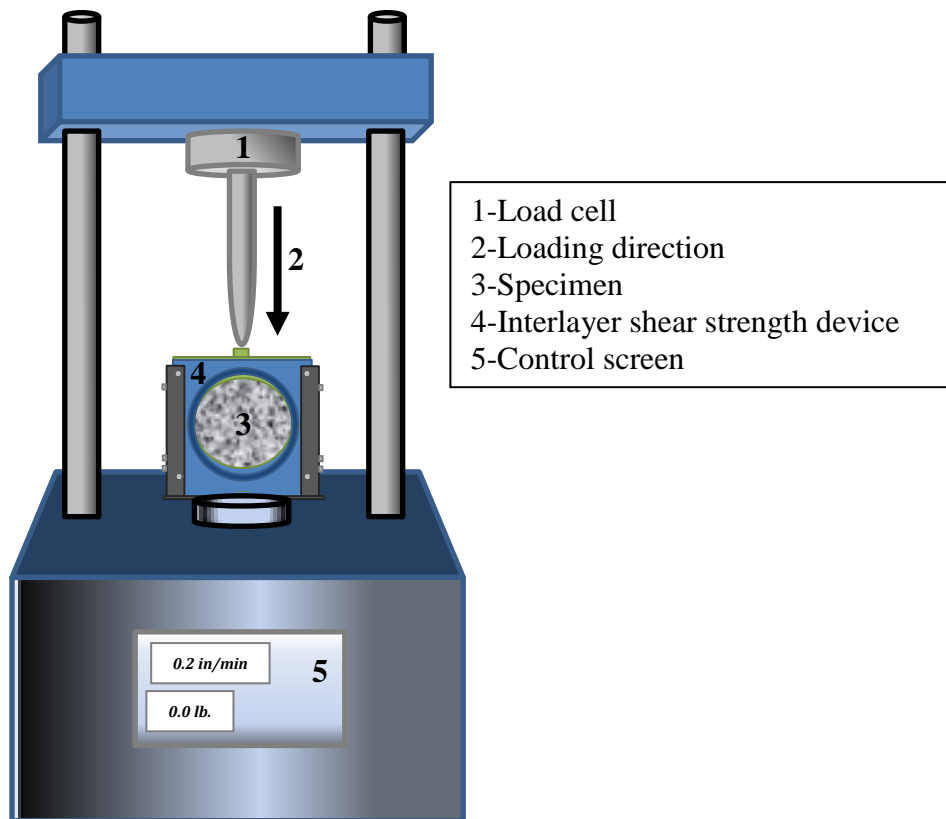
Figure 3 —Loading Frame with Shear Strength Device
