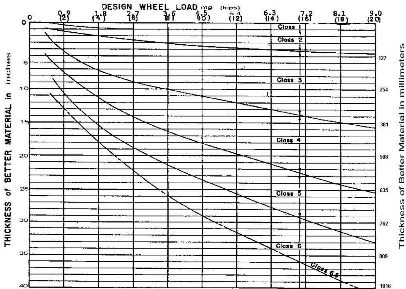
FLEXIBLE BASE DESIGN CHART
