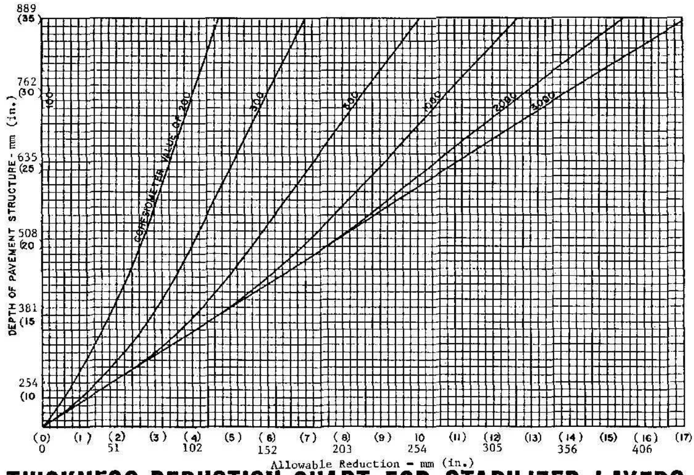
THICKNESS REDUCTION CHART FOR STABILIZED LAYERS
