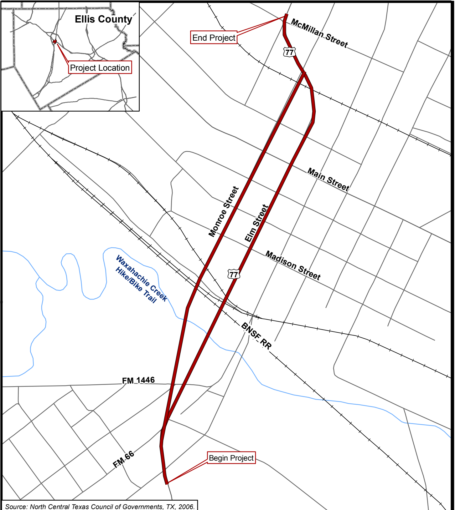
FIGURE 1 PROJECT LOCATION MAP US 77 FROM SOUTH OF FM 66 TO NORTH OF MCMILLAN STREET CSJ: 0048-03-050, 055
