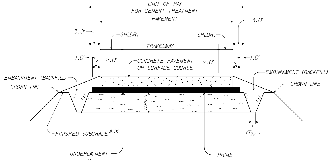
SECTION "C-C"
