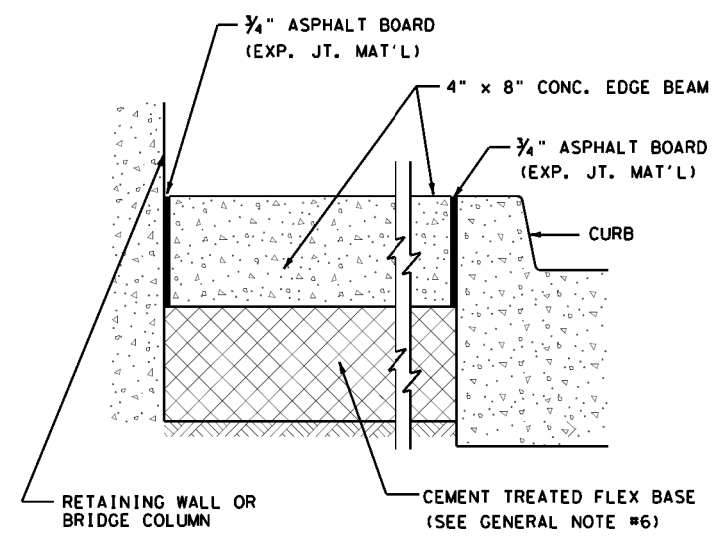
CONC. EDGE BEAM EXPANSION JOINT AT CURB, BRIDGE COLUMN OR RETAINING WALL (SECTION B-B) N. T. S.
