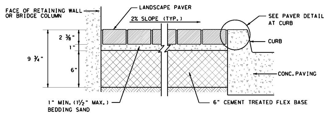
PAVER DETAIL AT CURB & AT BRIDGE COLUMN OR RETAINING WALL N. T. S.
