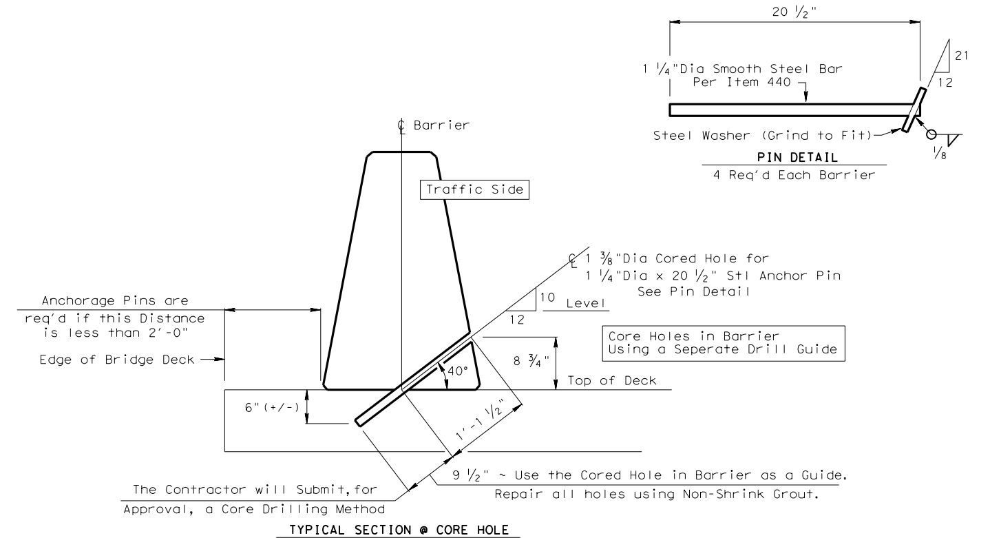
TYPICAL SECTION @ CORE HOLE
