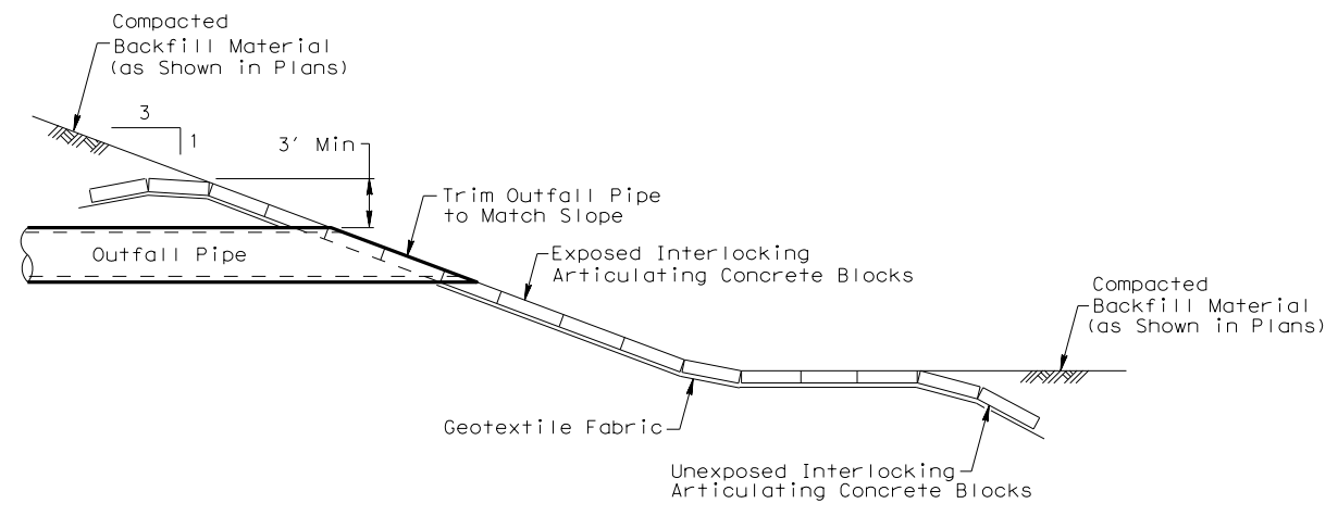
PIPE OUTLET DETAIL 1
