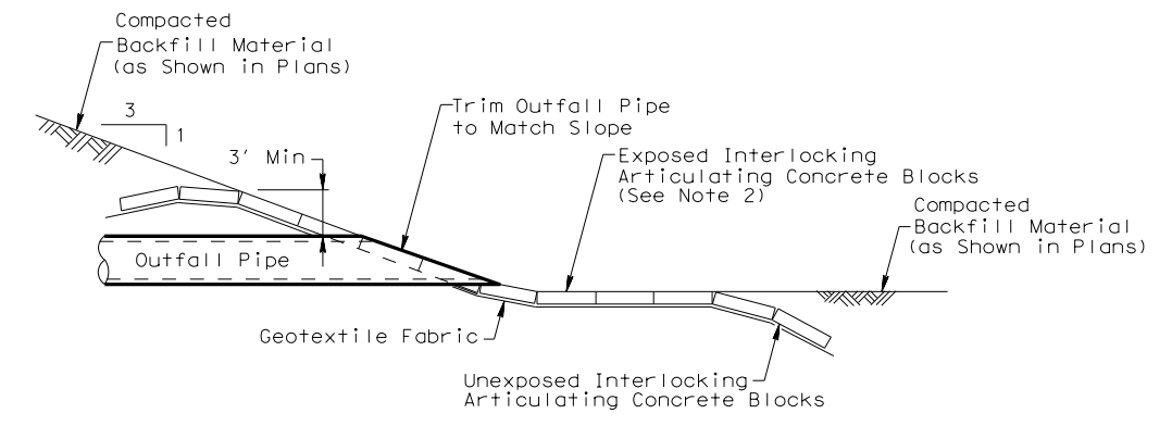
PIPE OUTLET DETAIL 2
