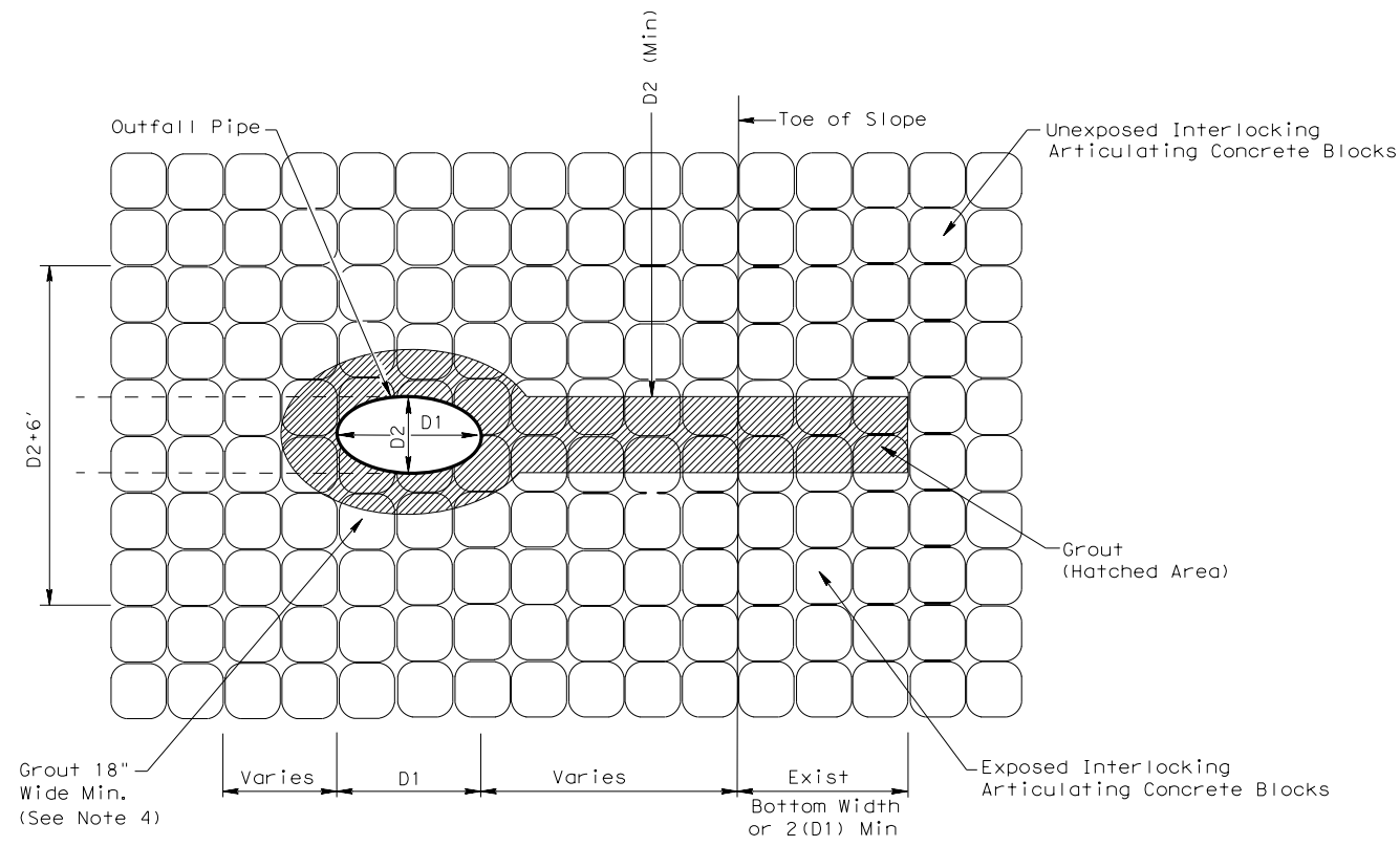
PLAN VIEW
