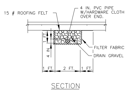
TYPE "B" WEEP HOLE
