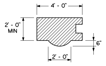
END COLUMN PLAN REQ'D AT ALL ENDS
