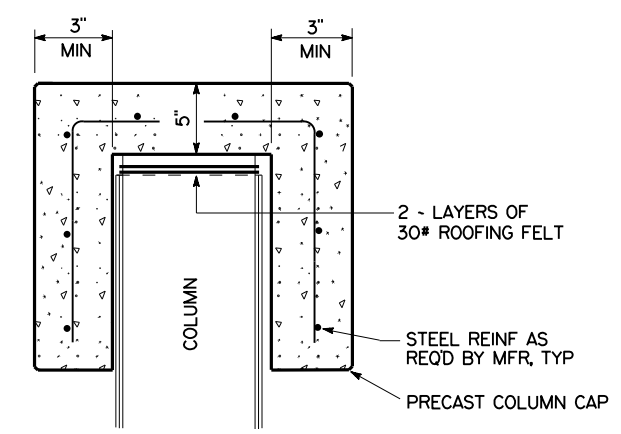
SECTION PRECAST CONCRETE COLUMN CAP
