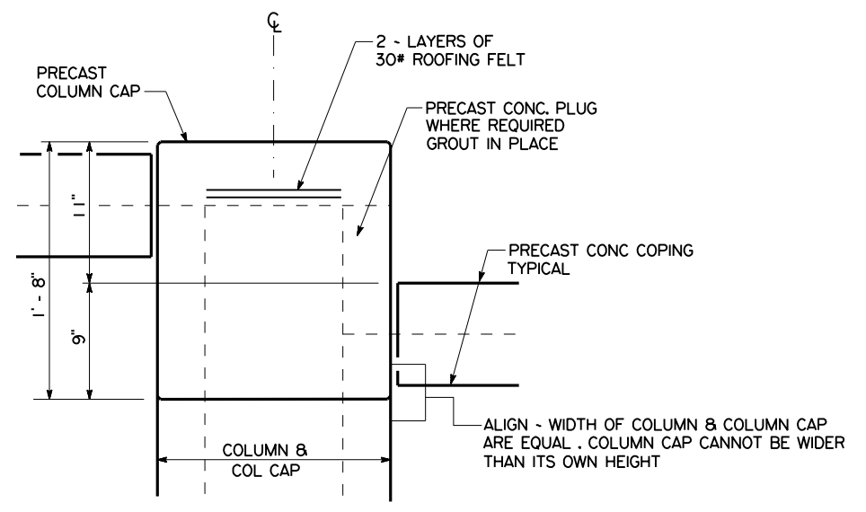
ELEVATION PRECAST CONCRETE COLUMN CAP
