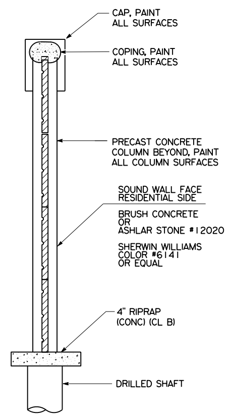
SECTION
