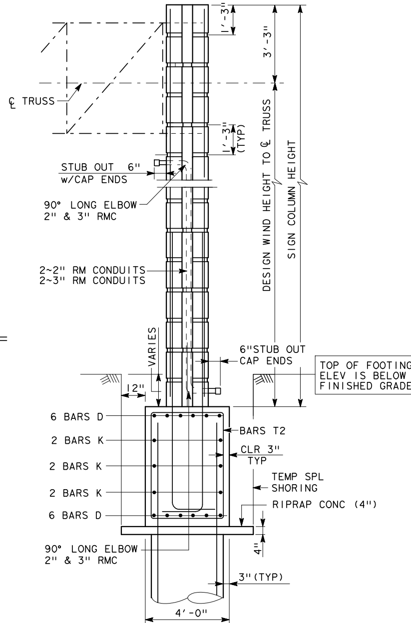
SIDE ELEVATION
