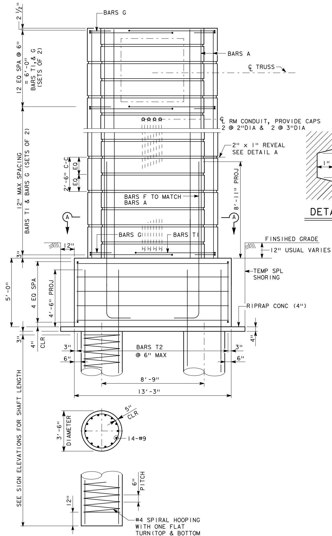
FRONT ELEVATION
