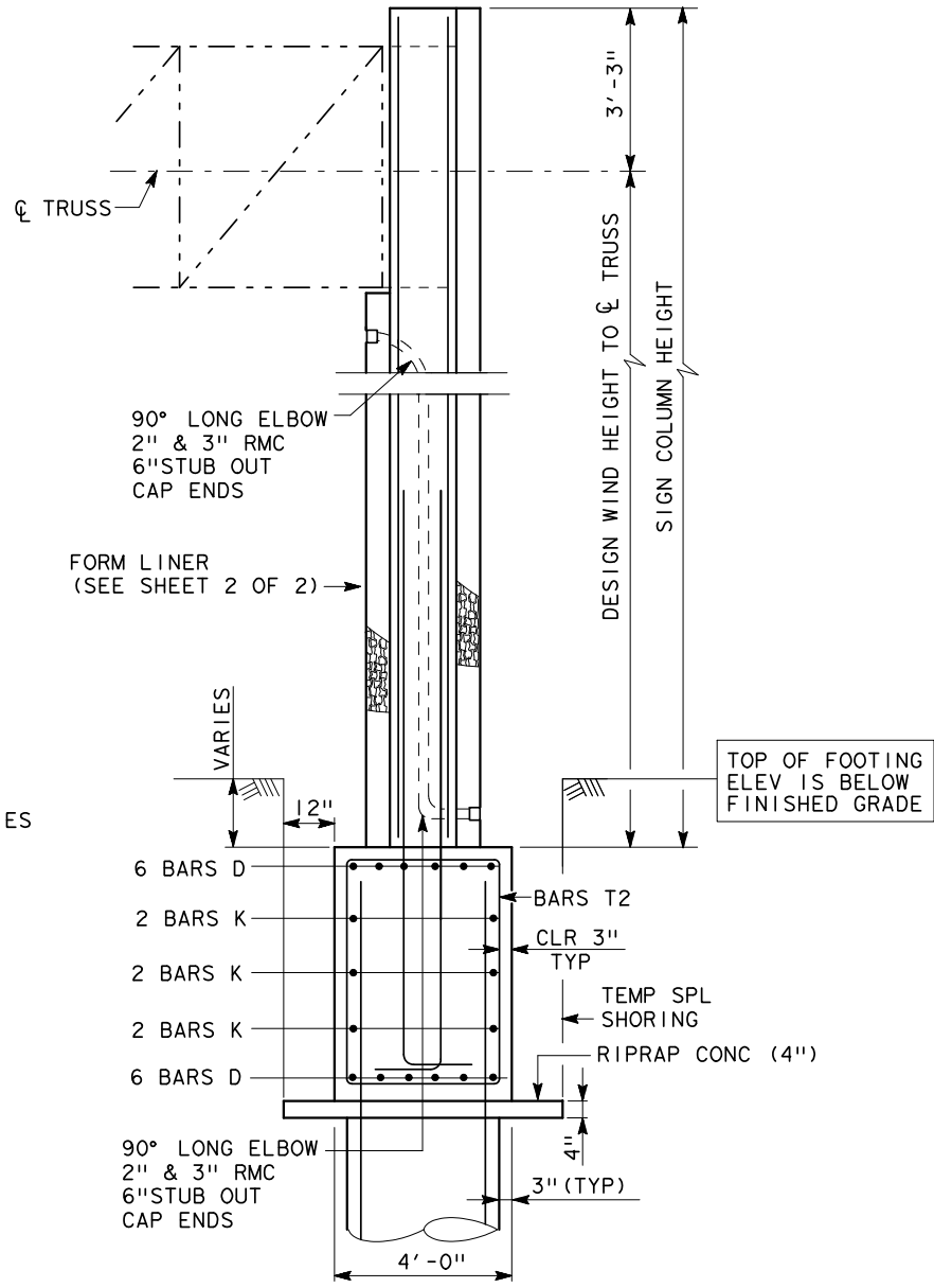
SIDE ELEVATION
