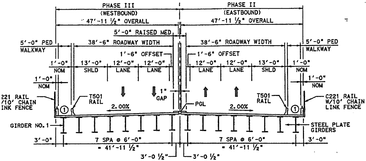
PROPOSED BRIDGE SECTION AT SPAN 6 (LOOKING UPSTATION)
