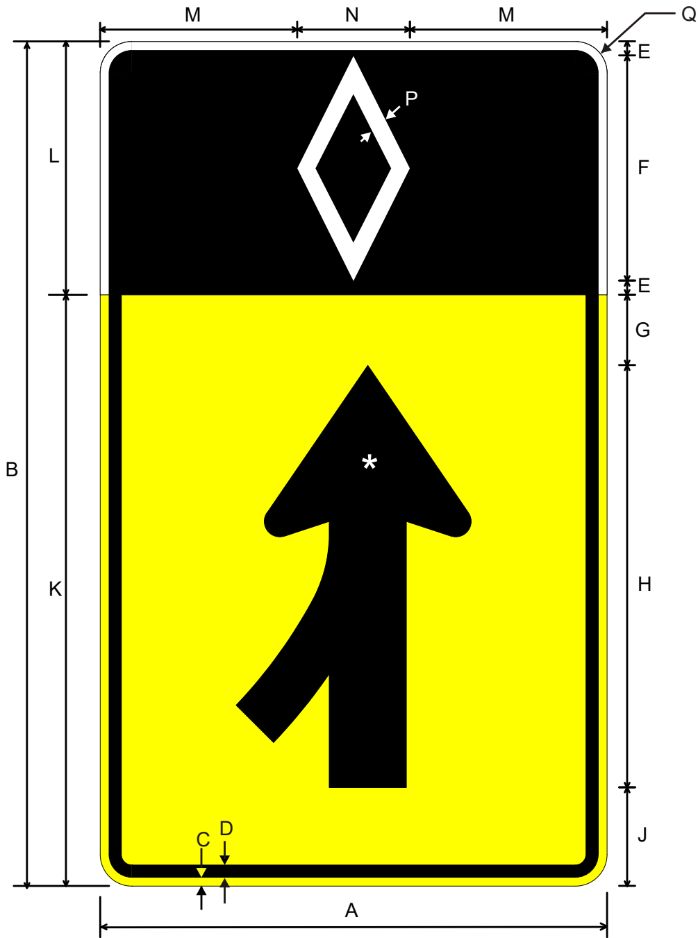
W4-1L (MODIFIED) HOV Merge (Symbol)
