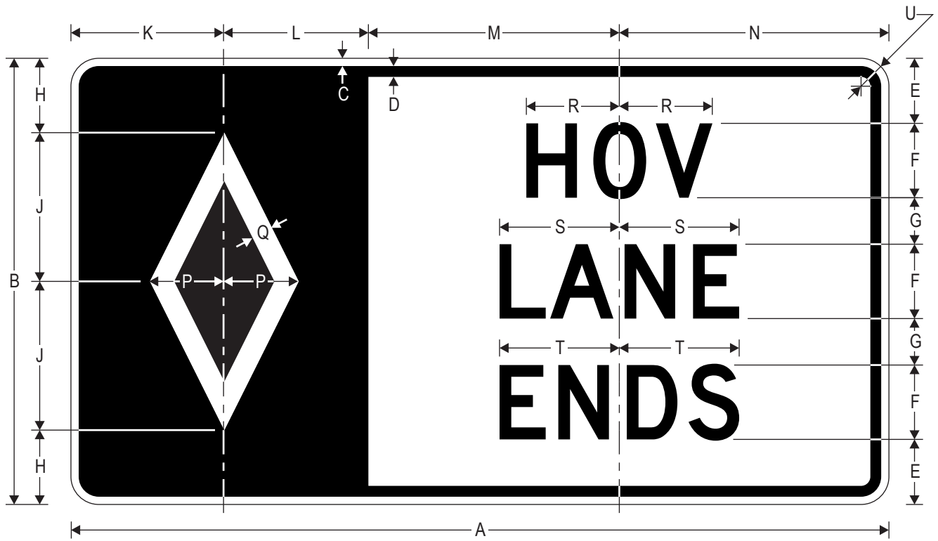
R3-15b (Overhead) HOV LANE ENDS ( with Symbol)
