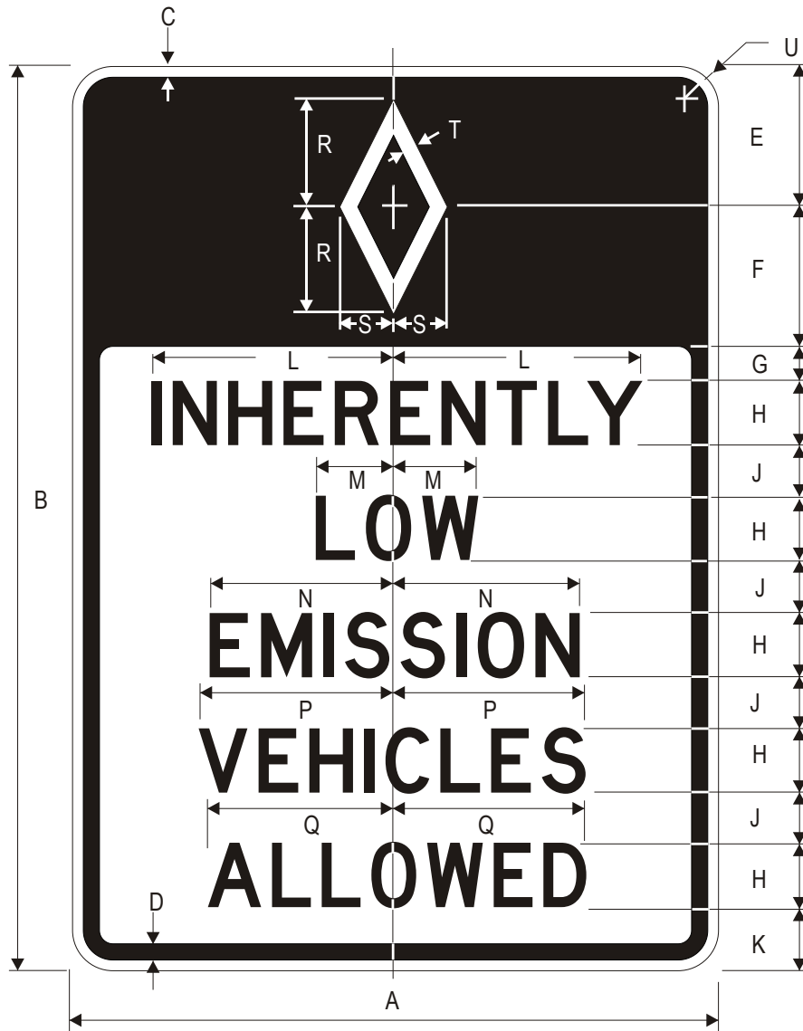
R3-10a (Post Mounted)
