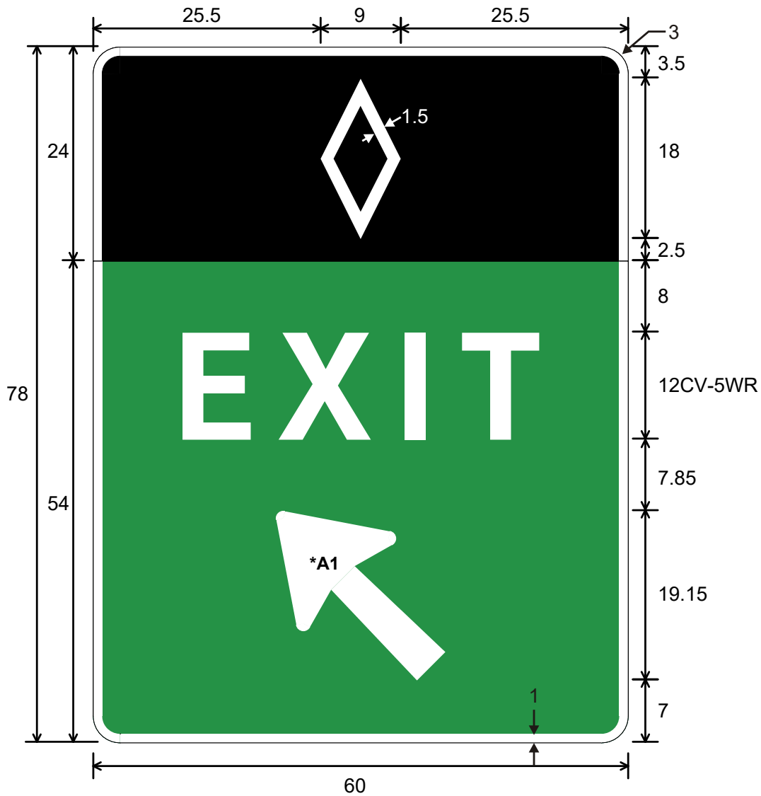
E8-4 Preferential Lane Direct Exit Gore
