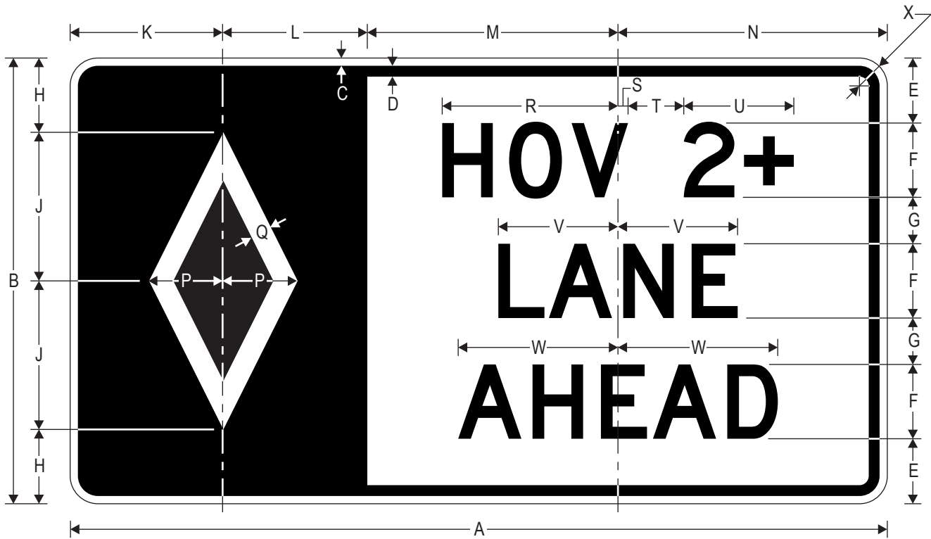
R3-15 (Overhead) HOV 2+ LANE AHEAD (with Symbol)
