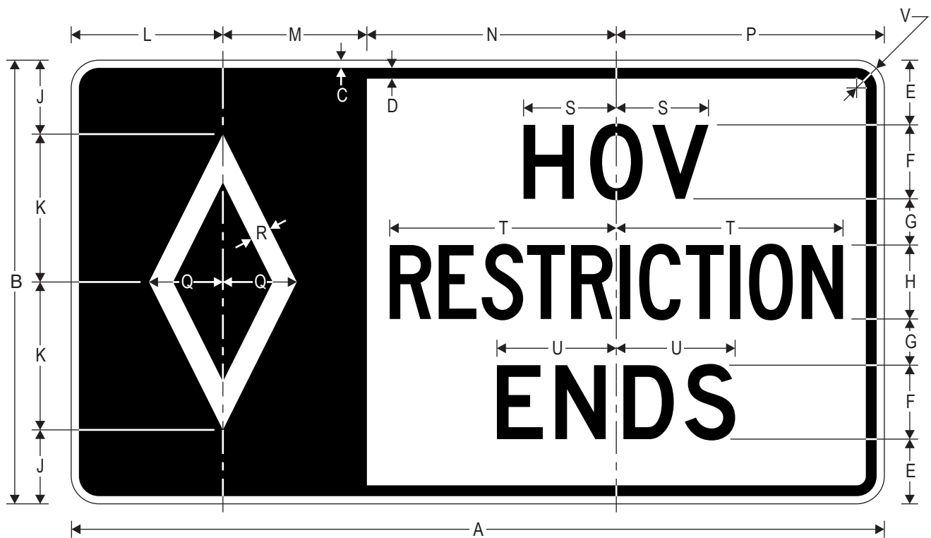
R3-15c (Overhead) HOV RESTRICTION ENDS (with Symbol)
