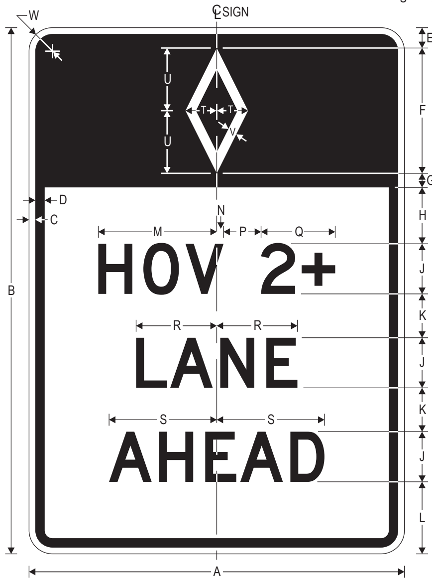
R3-12 (Post Mounted) HOV 2+ LANE AHEAD (with Symbol)
