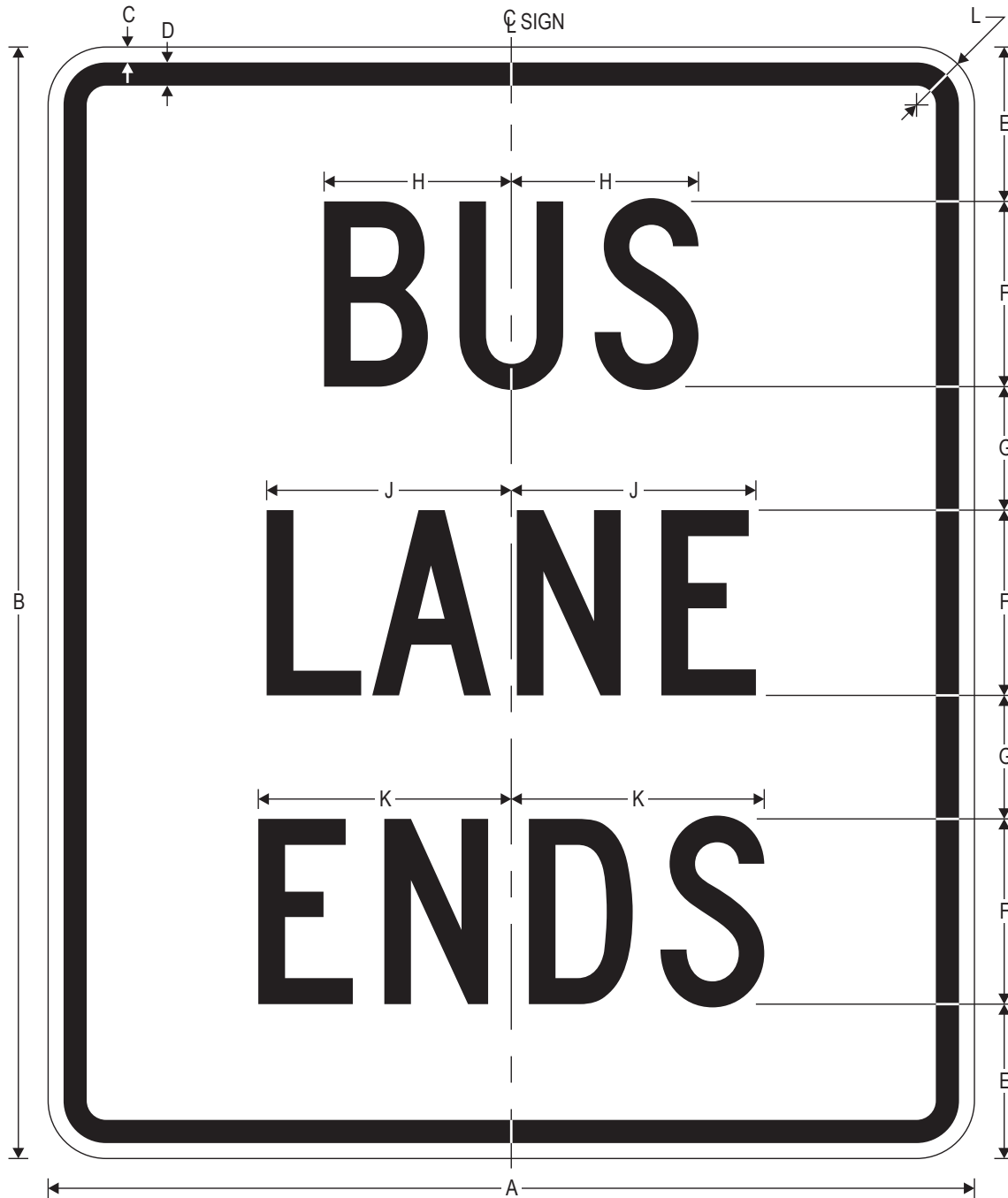
R3-12g BUS LANE ENDS
