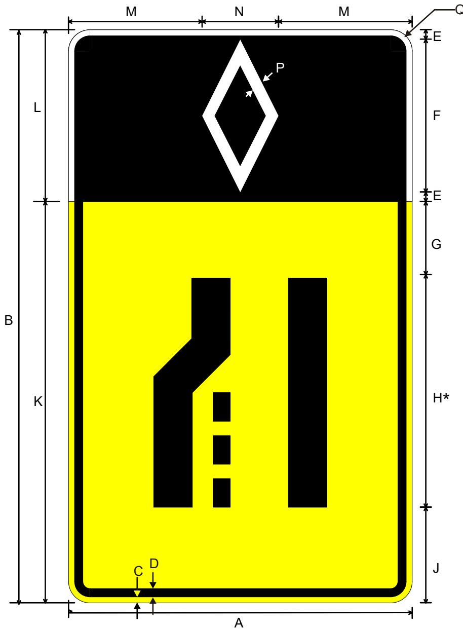
W4-2L (MODIFIED) HOV LANE ENDS (Symbol)
