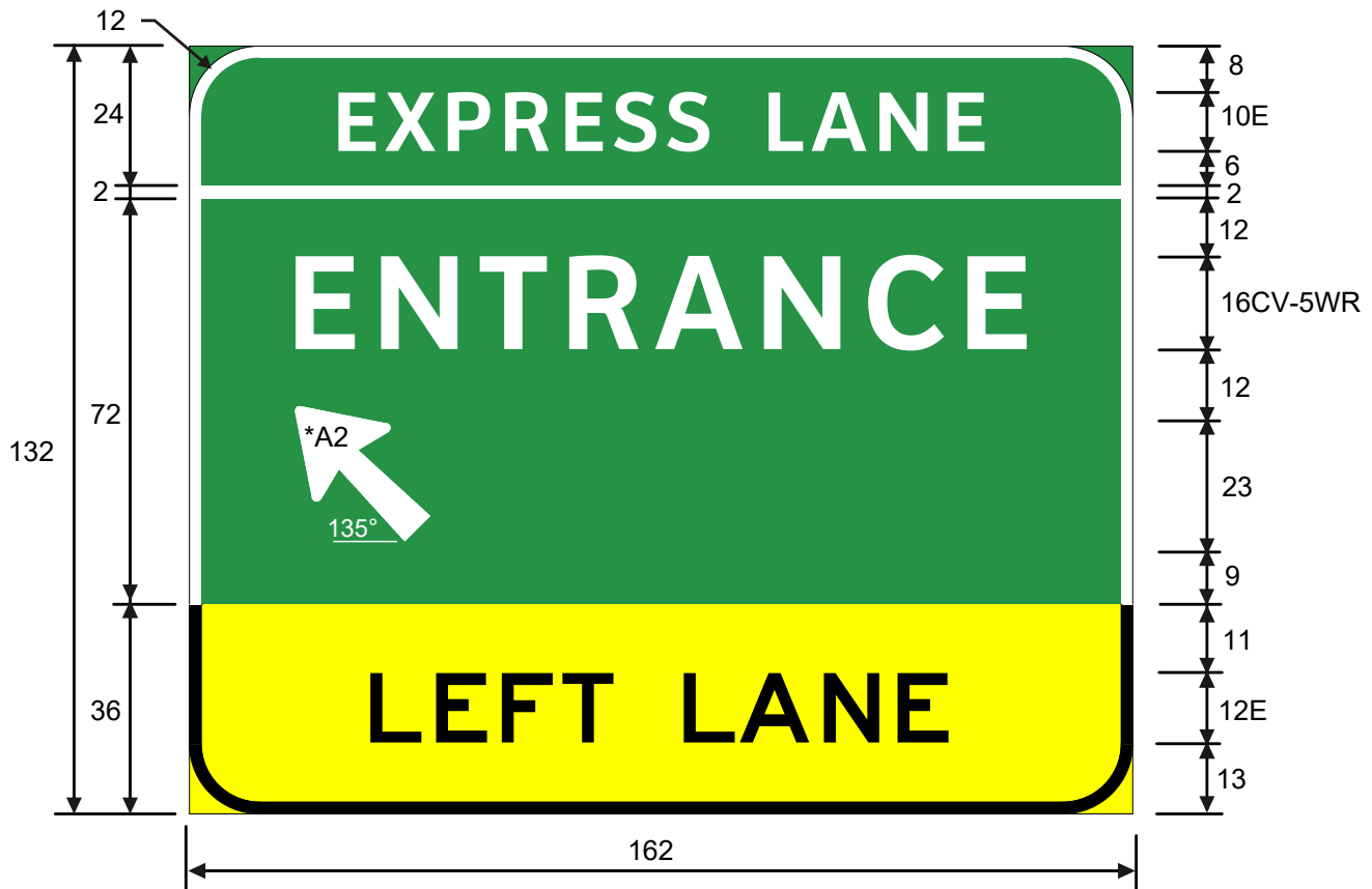
E8-2aT Advanced ENTRANCE LEFT LANE (45 Degree arrow)
