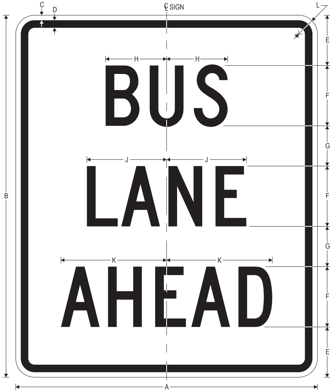
R3-12f BUS LANE AHEAD
