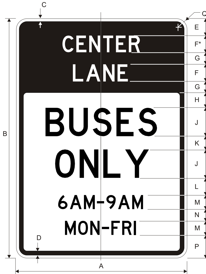
R3-11b (Post Mounted) CENTER LANE BUSES ONLY
