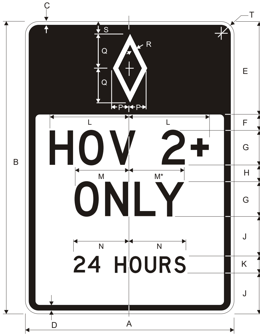
R3-11c (Post Mounted)
