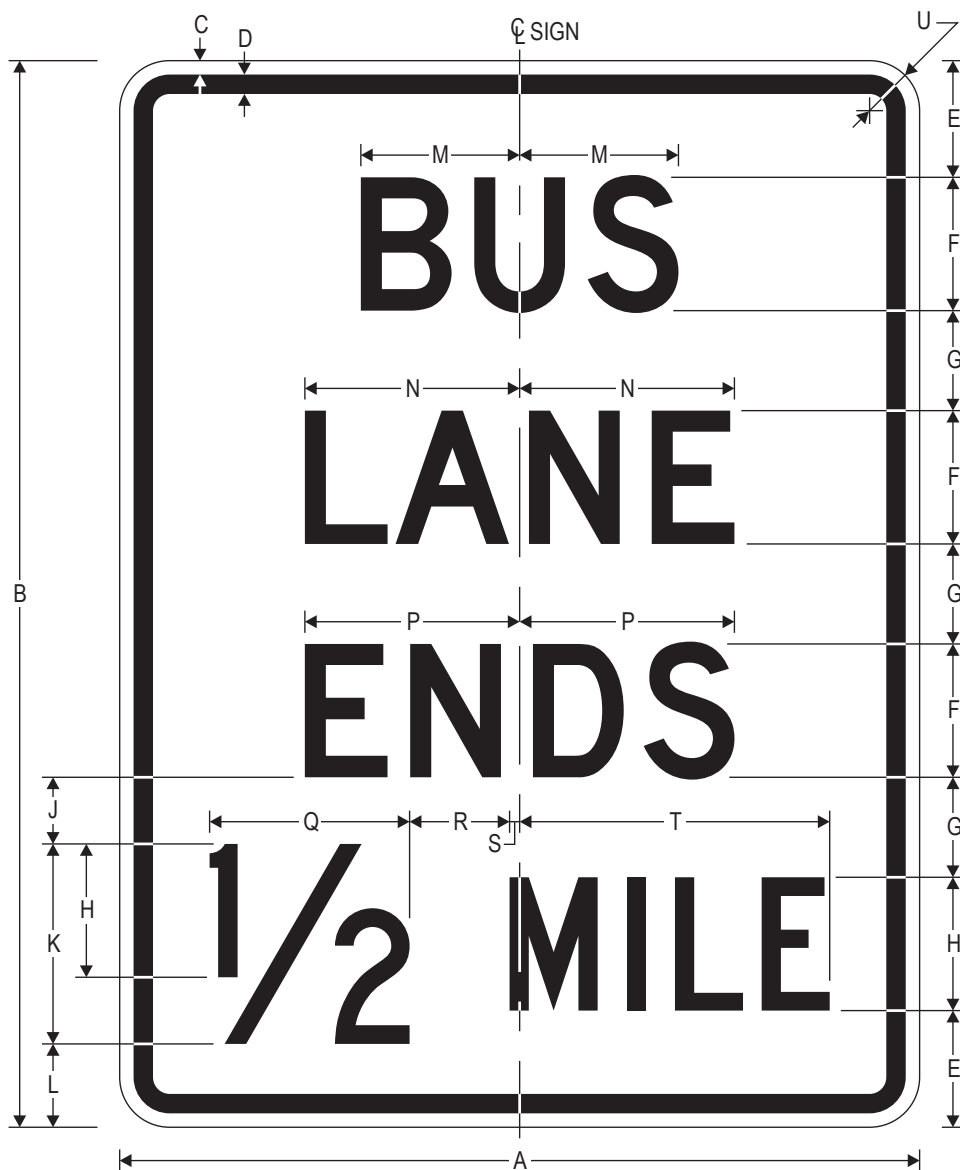
R3-12h BUS LANE ENDS X MILE
