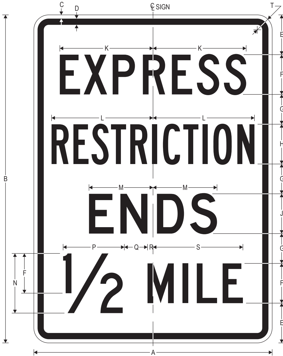
R3-42c (Post Mounted) EXPRESS RESTRICTION ENDS X MILE
