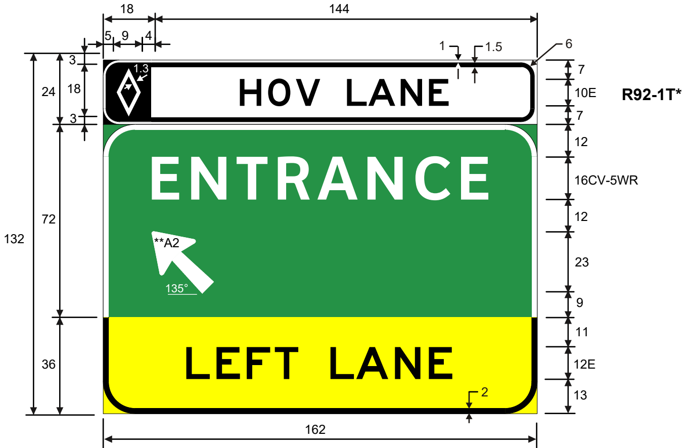
E8-2T Advanced ENTRANCE LEFT LANE (45 Degree arrow)
