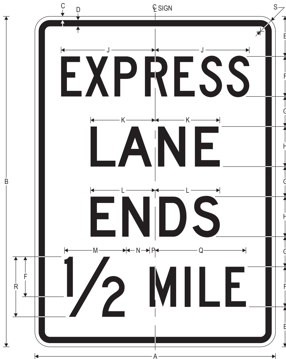
R3-42a (Post Mounted) EXPRESS LANE ENDS X MILE
