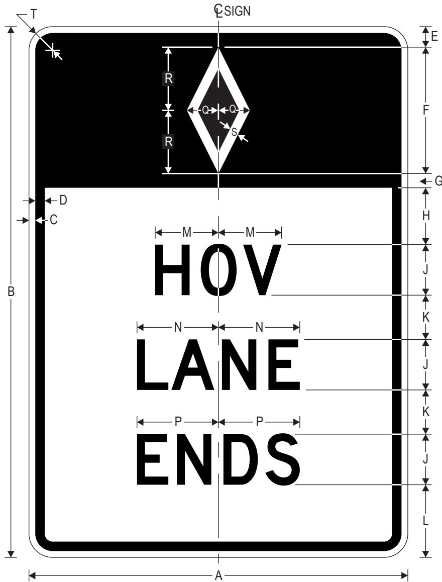
R3-12a (Post Mounted) HOV LANE ENDS (with Symbol)
