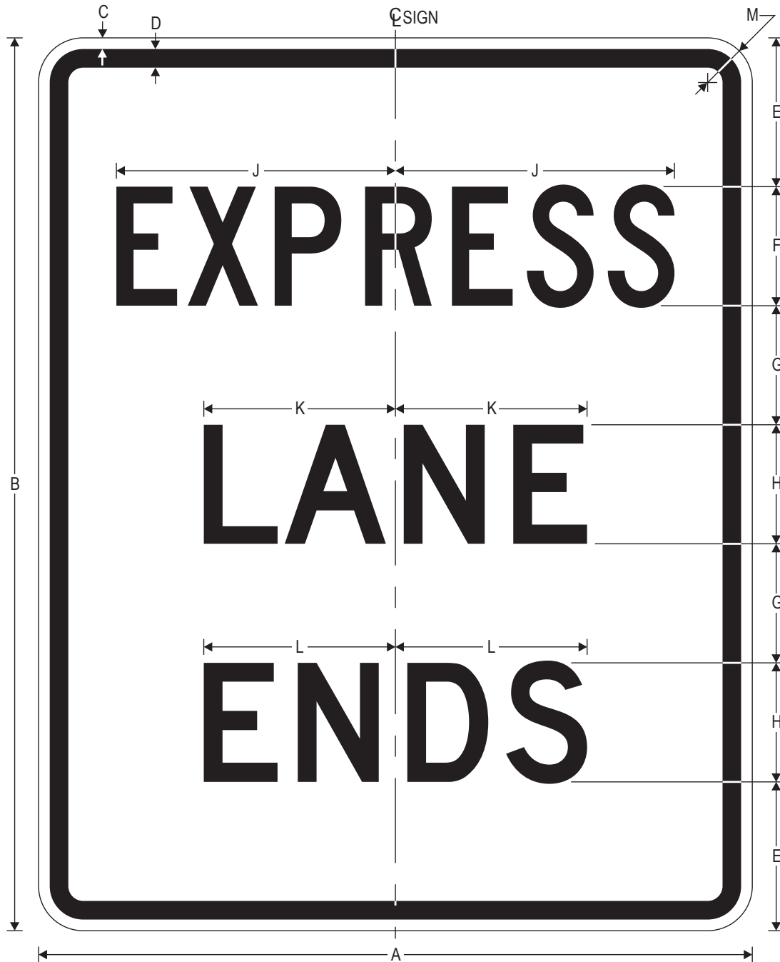
R3-42 (Post Mounted) EXPRESS LANE ENDS
