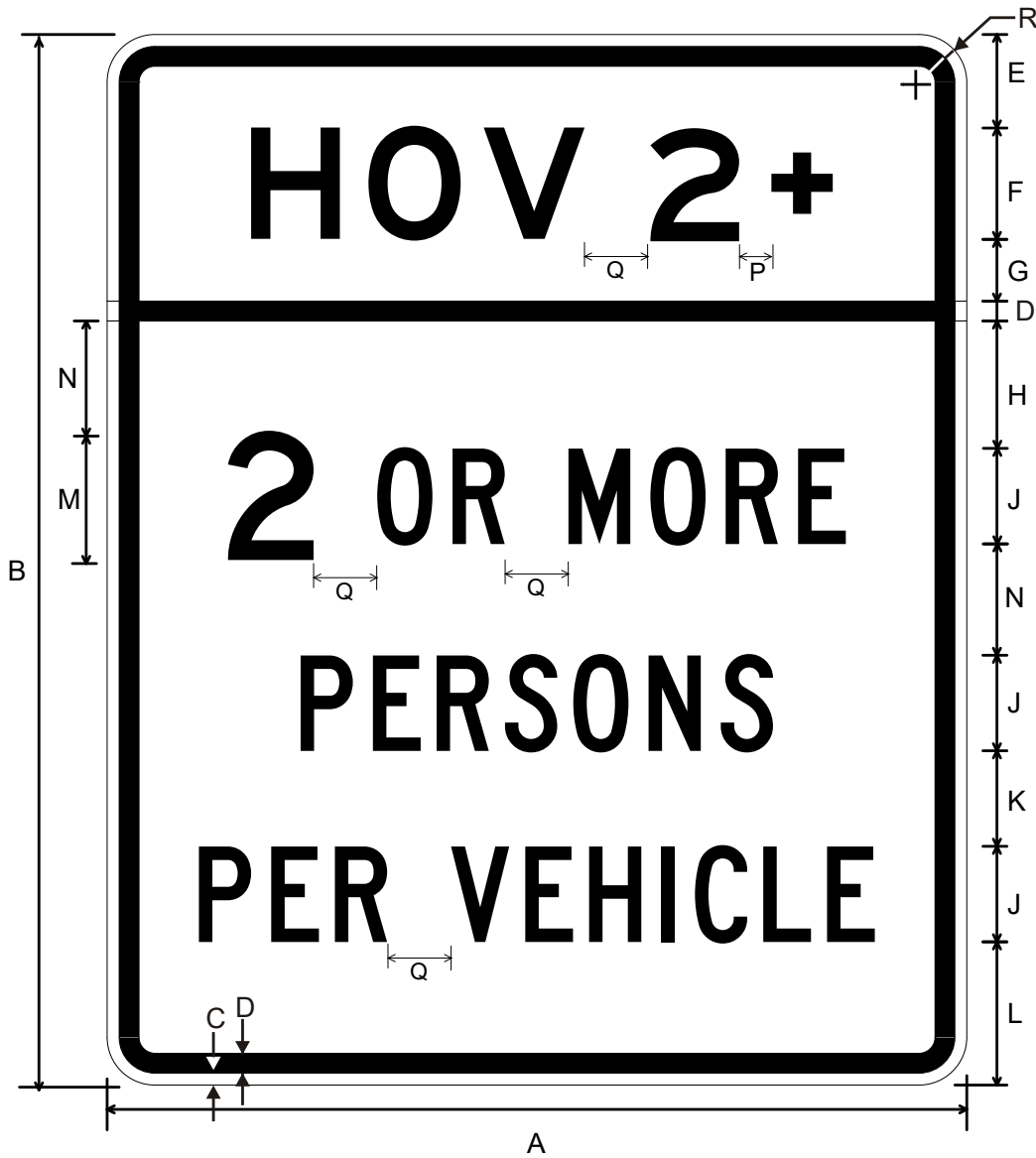
R3-40T (Post Mounted) HOV 2+ 2 OR MORE PERSONS PER VEHICLE
