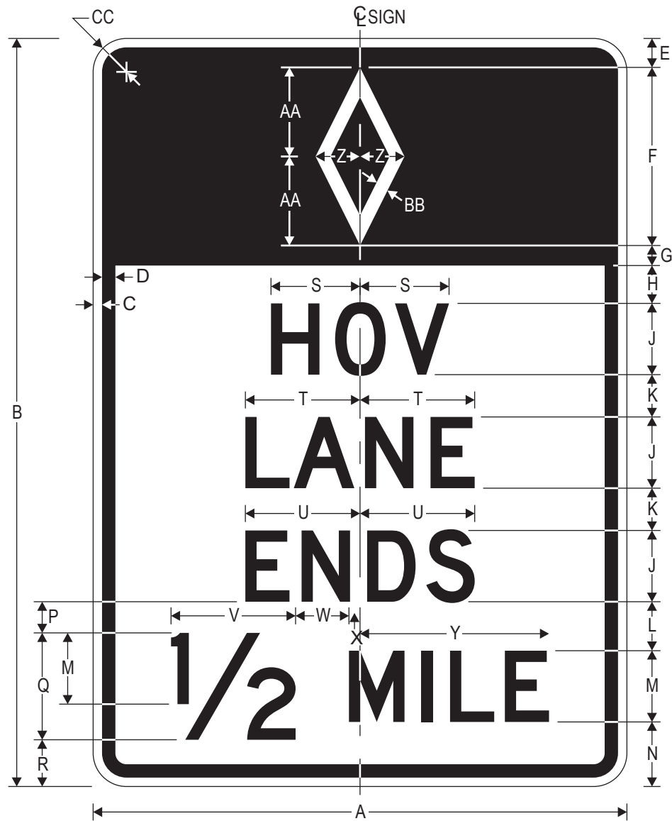
R3-12b (Post Mounted) HOV LANE ENDS X MILE (with Symbol)
