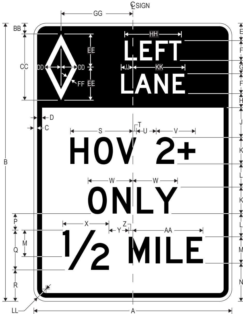
R3-12e (Post Mounted)
