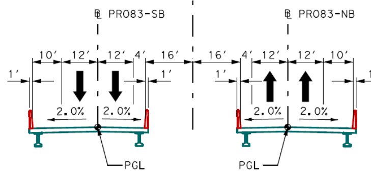
PROPOSED US 83 BRIDGE TYPICAL SECTION
