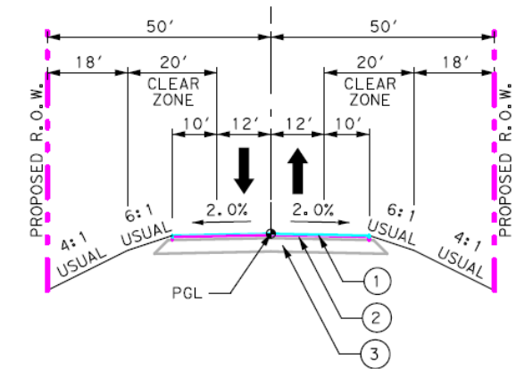
PROPOSED FM 3034 TYPICAL SECTION
