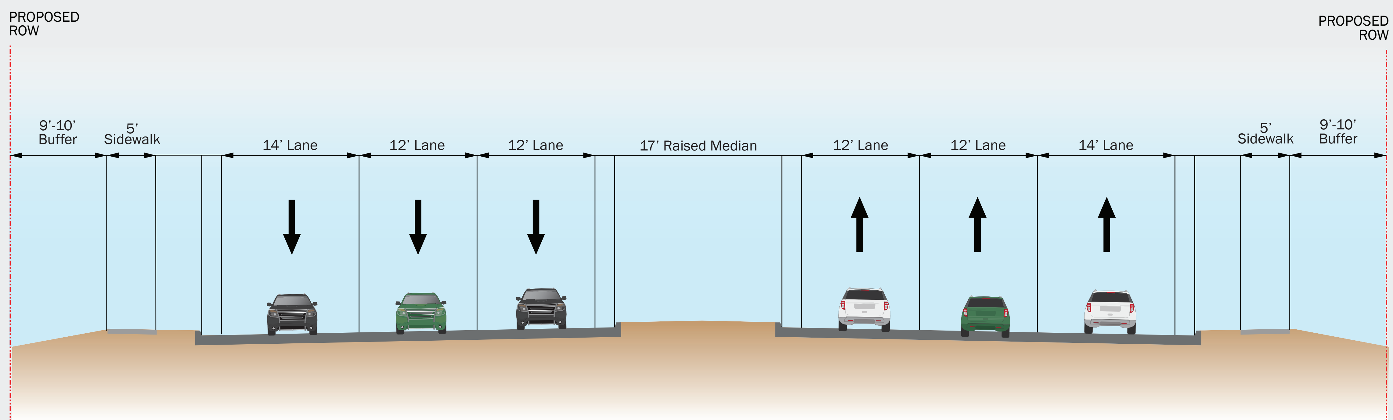
Proposed FM 1515
