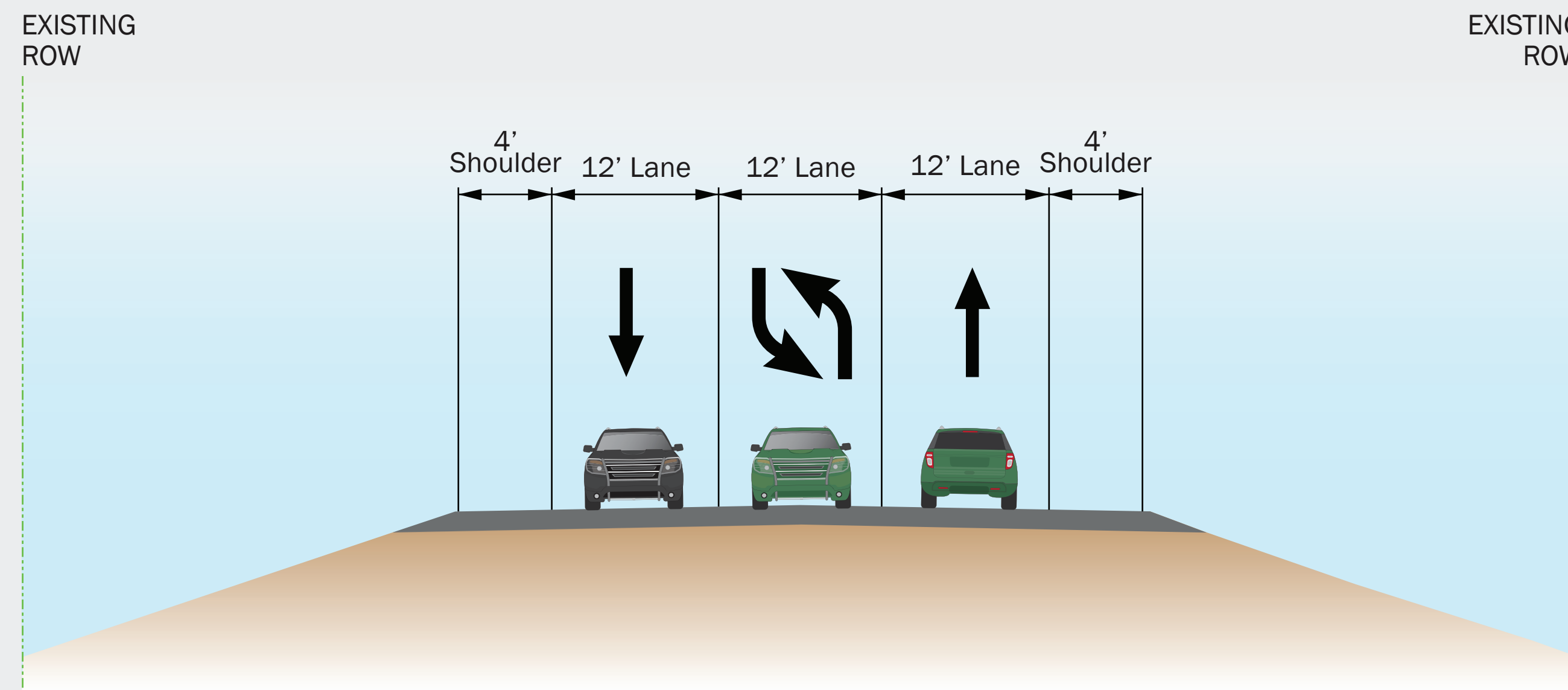
Existing FM 1515
