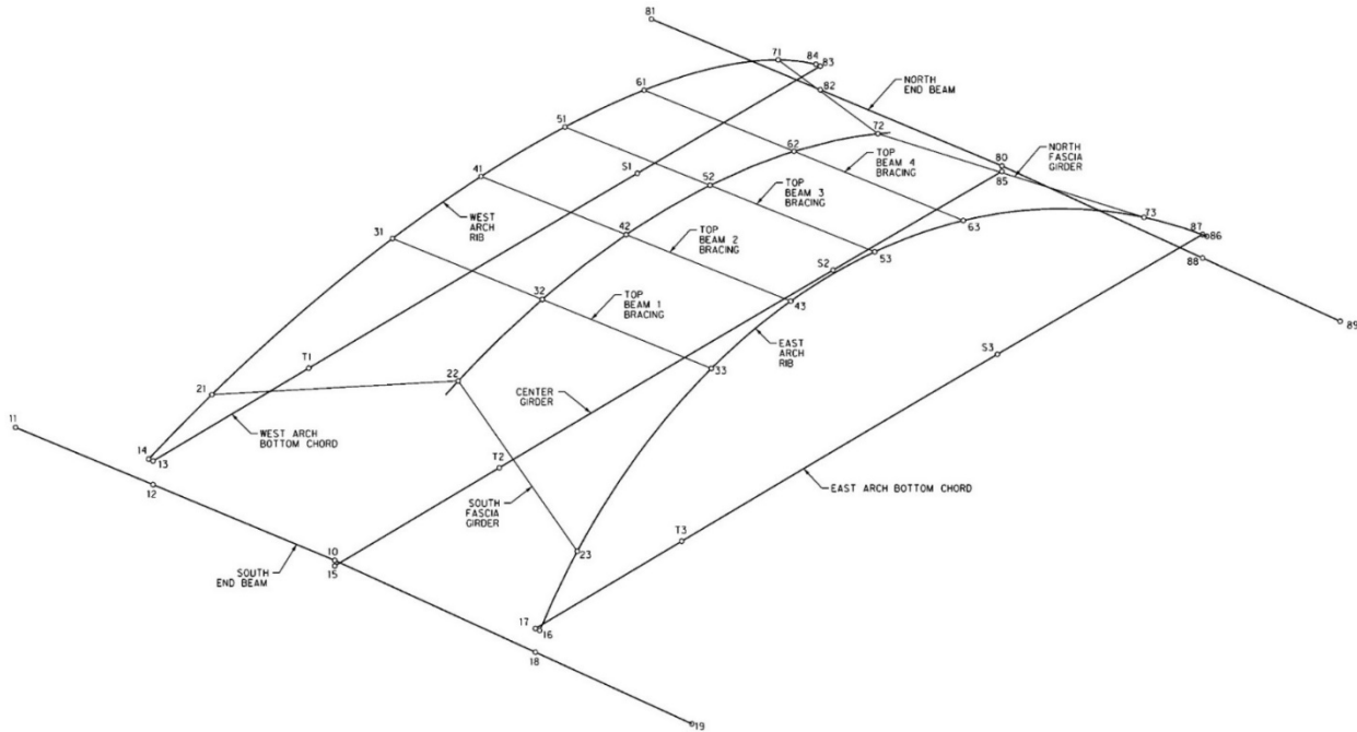
Figure 1: Bridge Frame
